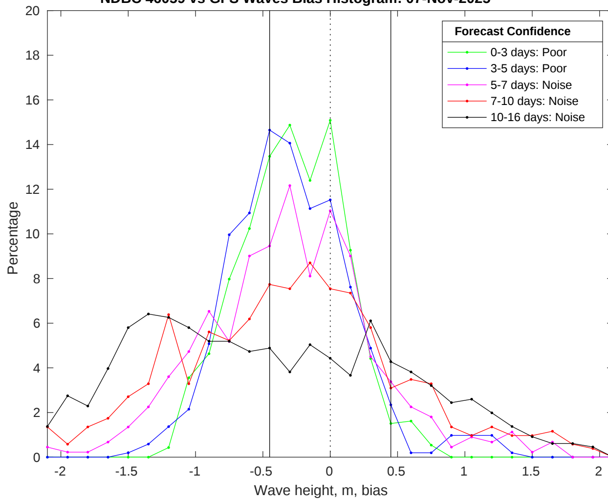
NDBC 46059 vs GFS Waves Bias Histogram: 07-Nov-2025
