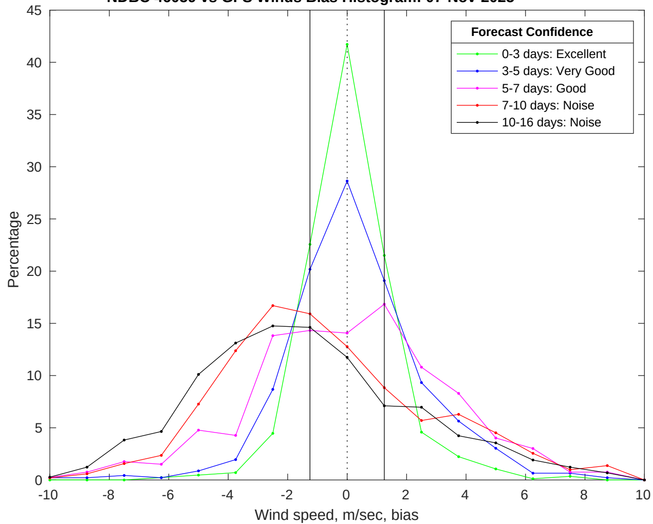
NDBC 46059 vs GFS Winds Bias Histogram: 07-Nov-2025
