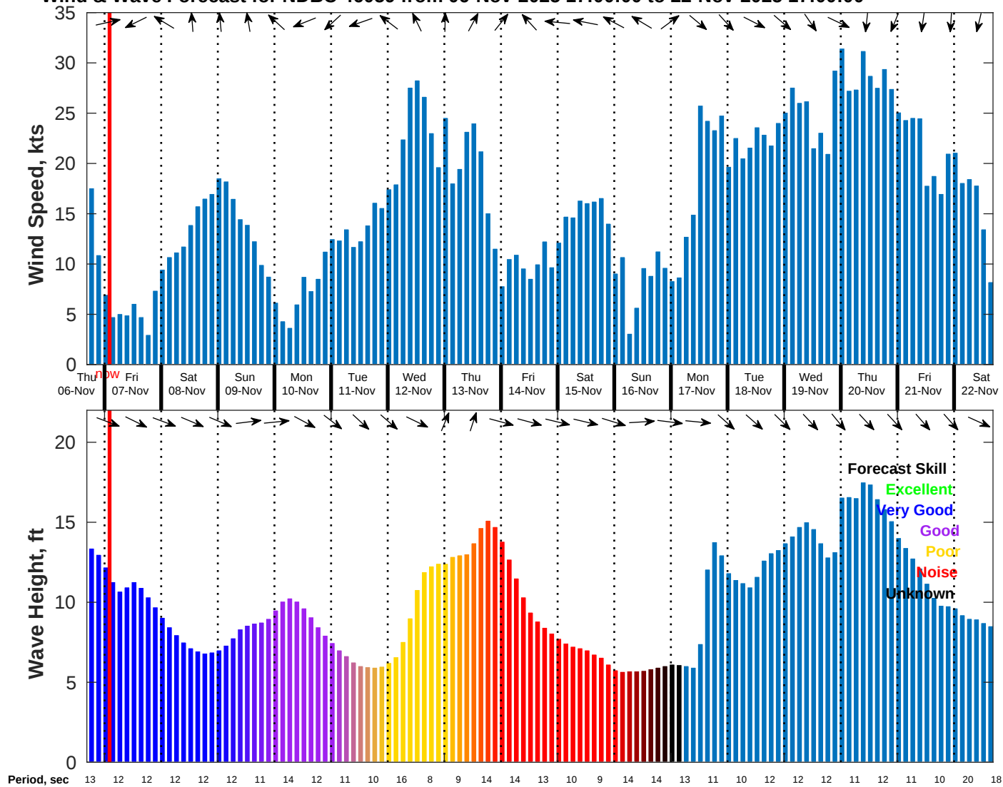
Wind & Wave Forecast for NDBC 46059 from 06-Nov-2025 17:00:00 to 22-Nov-2025 17:00:00
