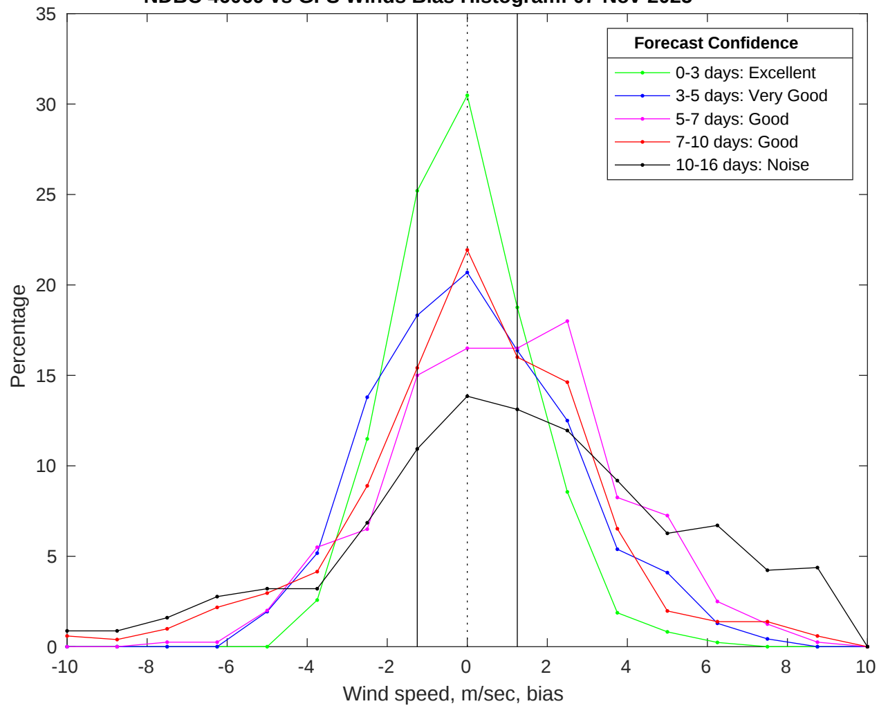
NDBC 46069 vs GFS Winds Bias Histogram: 07-Nov-2025
