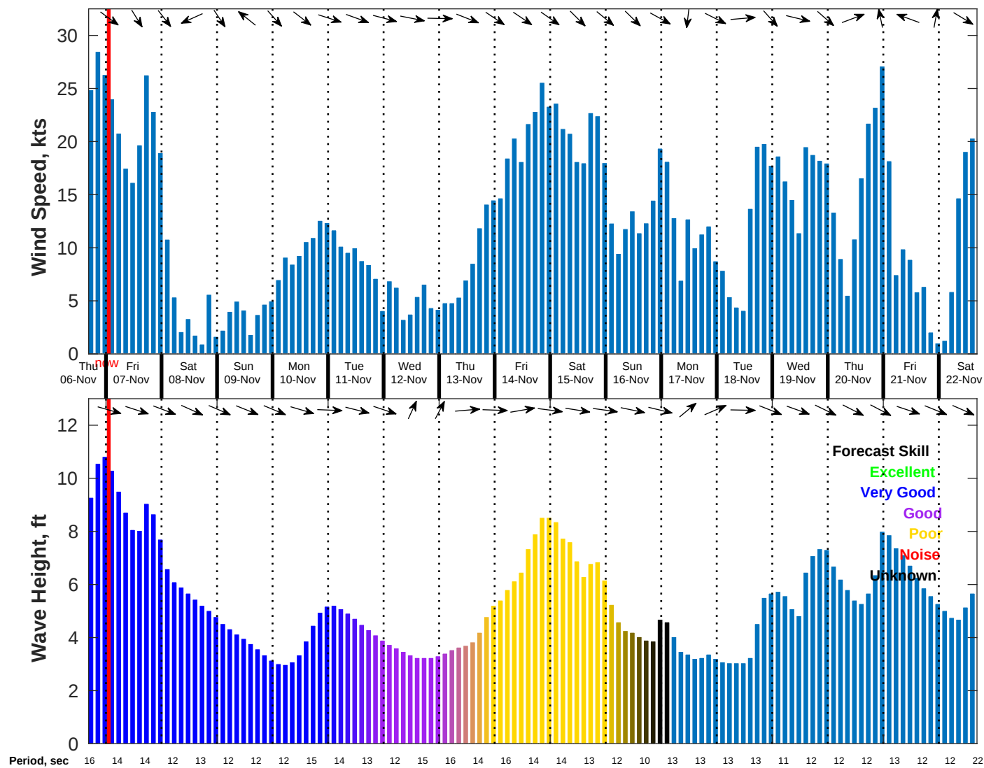
Wind & Wave Forecast for NDBC 46069 from 06-Nov-2025 16:00:00 to 22-Nov-2025 16:00:00
