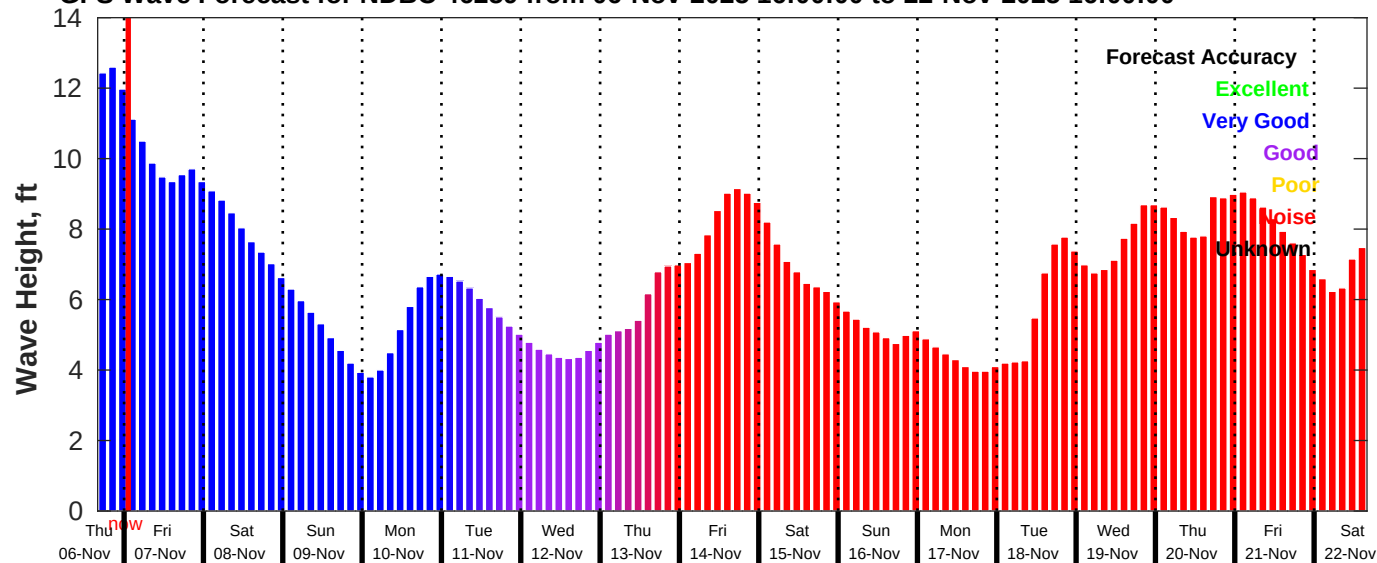
GFS Wave Forecast for NDBC 46259 from 06-Nov-2025 16:00:00 to 22-Nov-2025 16:00:00
