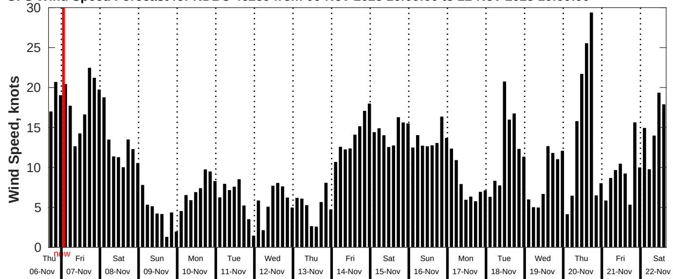
GFS Wind Speed Forecast for NDBC 46259 from 06-Nov-2025 16:00:00 to 22-Nov-2025 16:00:00
