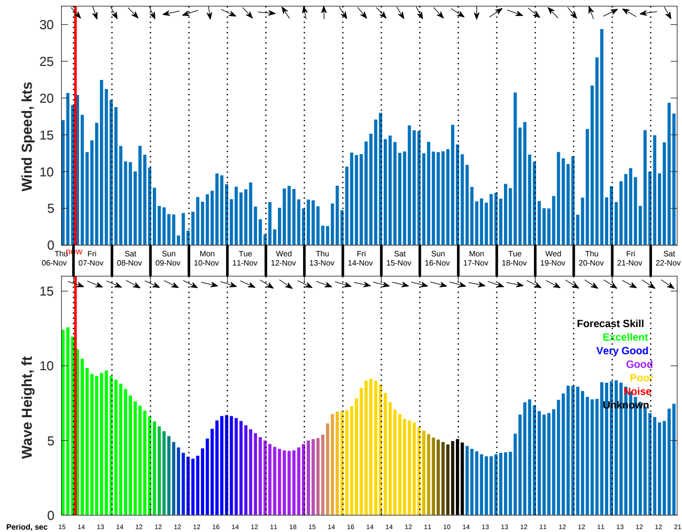
Wind & Wave Forecast for NDBC 46259 from 06-Nov-2025 16:00:00 to 22-Nov-2025 16:00:00
