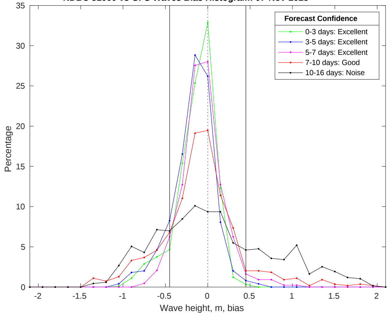
NDBC 51000 vs GFS Waves Bias Histogram: 07-Nov-2025
