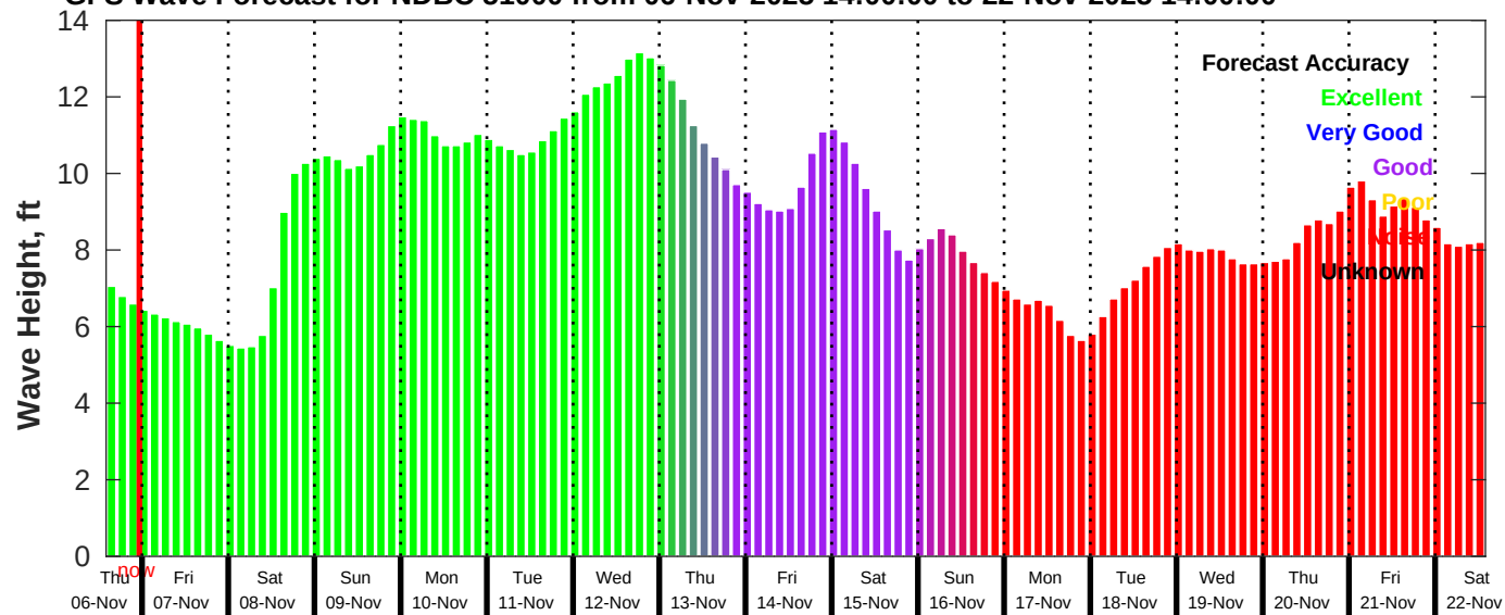
GFS Wave Forecast for NDBC 51000 from 06-Nov-2025 14:00:00 to 22-Nov-2025 14:00:00
