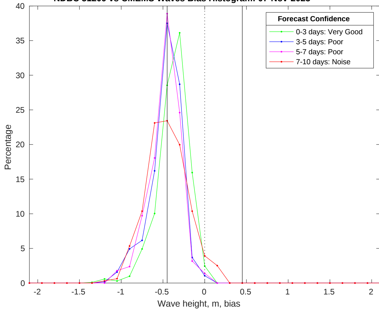
NDBC 51209 vs CMEMS Waves Bias Histogram: 07-Nov-2025
