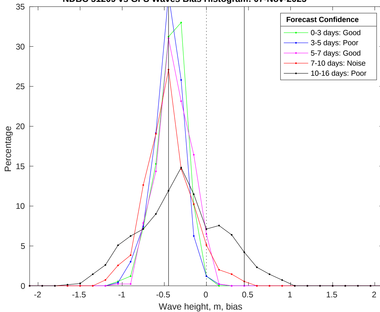
NDBC 51209 vs GFS Waves Bias Histogram: 07-Nov-2025
