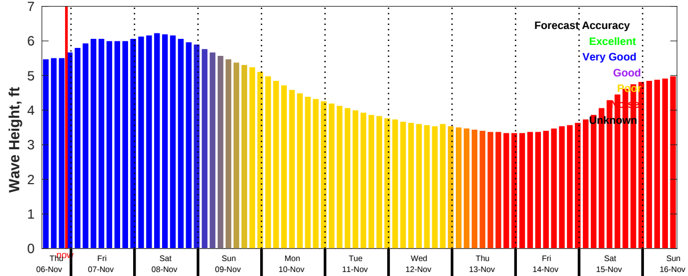
CMEMS Wave Forecast for NDBC 51209 from 06-Nov-2025 13:00:00 to 16-Nov-2025 13:00:00
