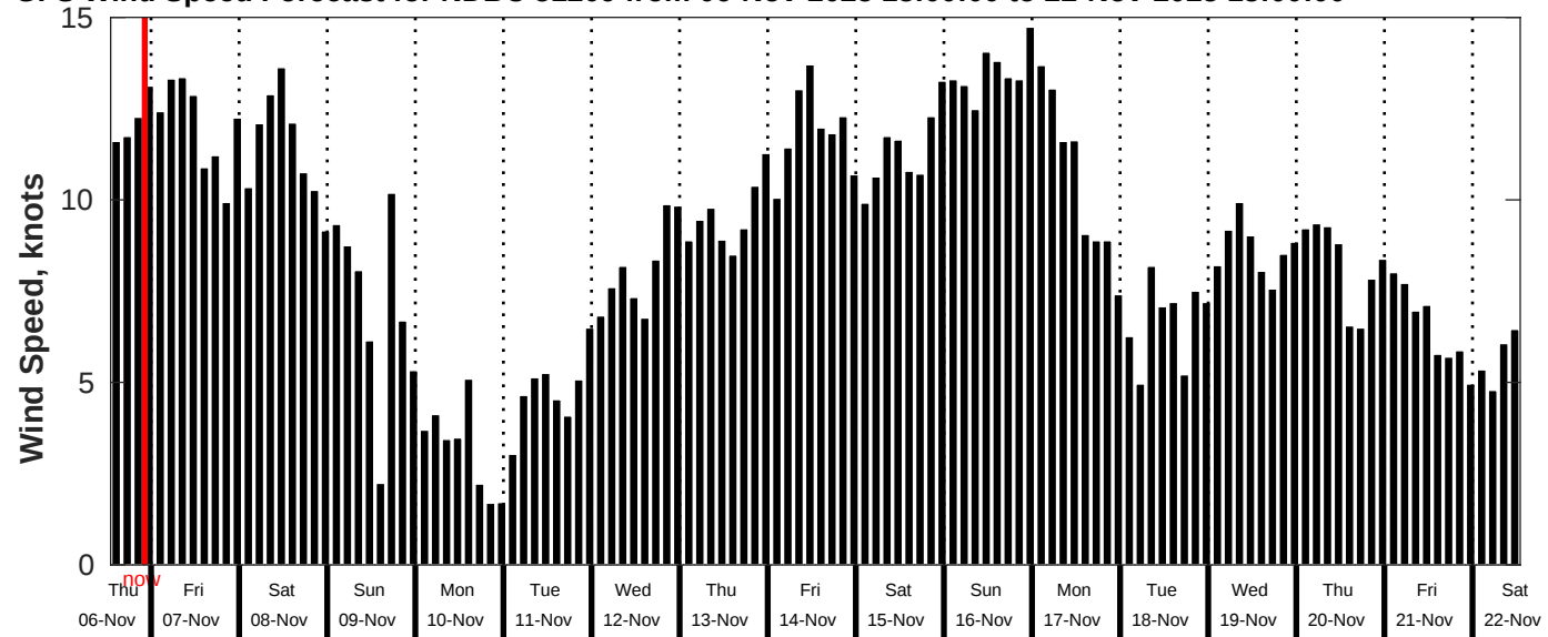
GFS Wind Speed Forecast for NDBC 51209 from 06-Nov-2025 13:00:00 to 22-Nov-2025 13:00:00
