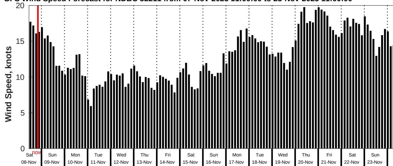
GFS Wind Speed Forecast for NDBC 52211 from 07-Nov-2025 11:00:00 to 23-Nov-2025 11:00:00
