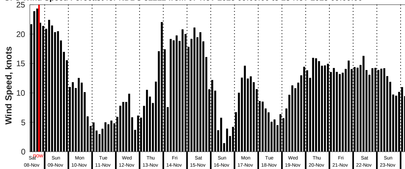
GFS Wind Speed Forecast for NDBC 52212 from 07-Nov-2025 09:00:00 to 23-Nov-2025 09:00:00
