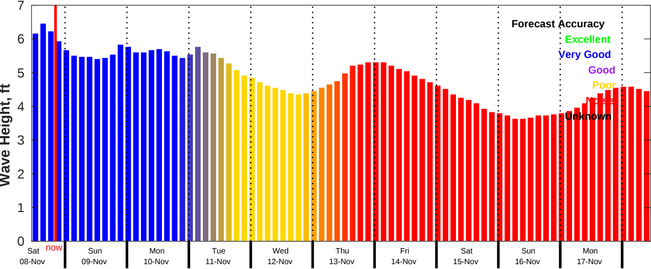
CMEMS Wave Forecast for NDBC 52213 from 07-Nov-2025 11:00:00 to 17-Nov-2025 11:00:00
