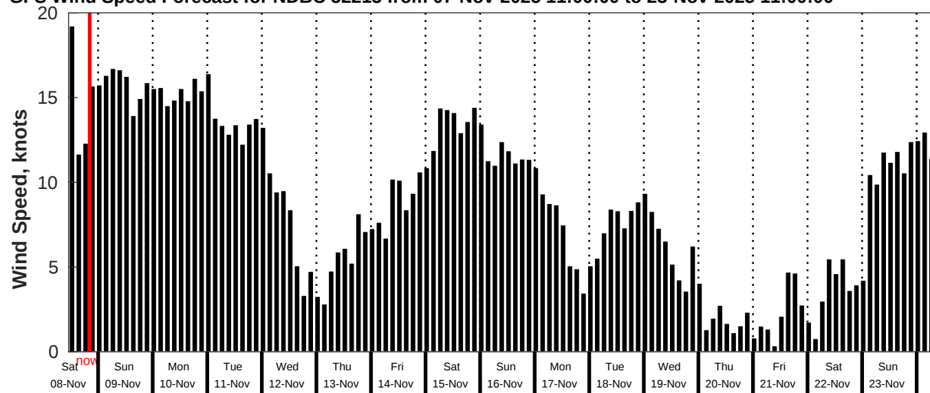
GFS Wind Speed Forecast for NDBC 52213 from 07-Nov-2025 11:00:00 to 23-Nov-2025 11:00:00
