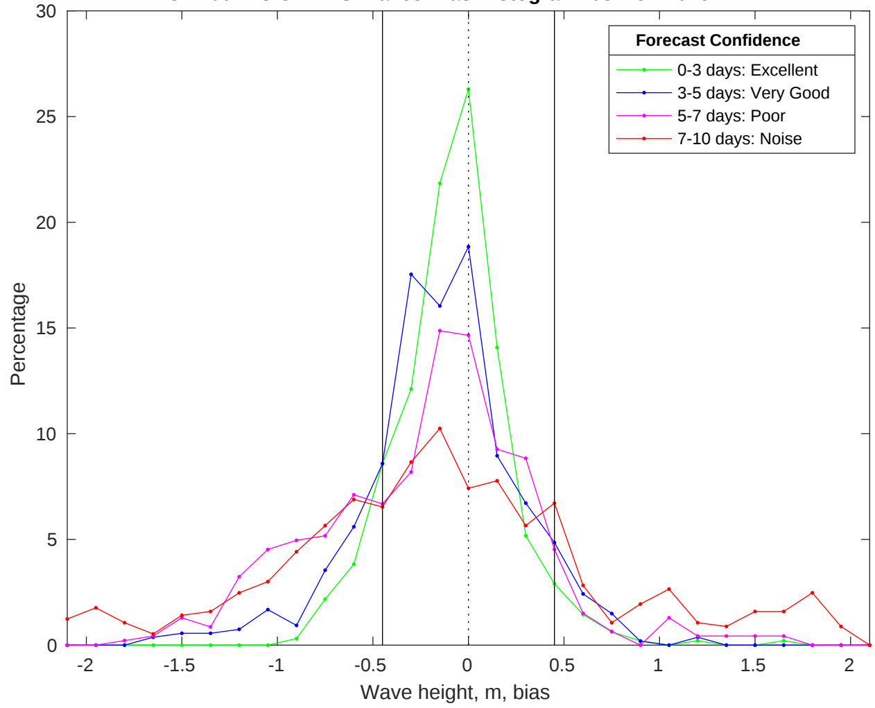
NDBC 41004 vs CMEMS Waves Bias Histogram: 08-Nov-2025
