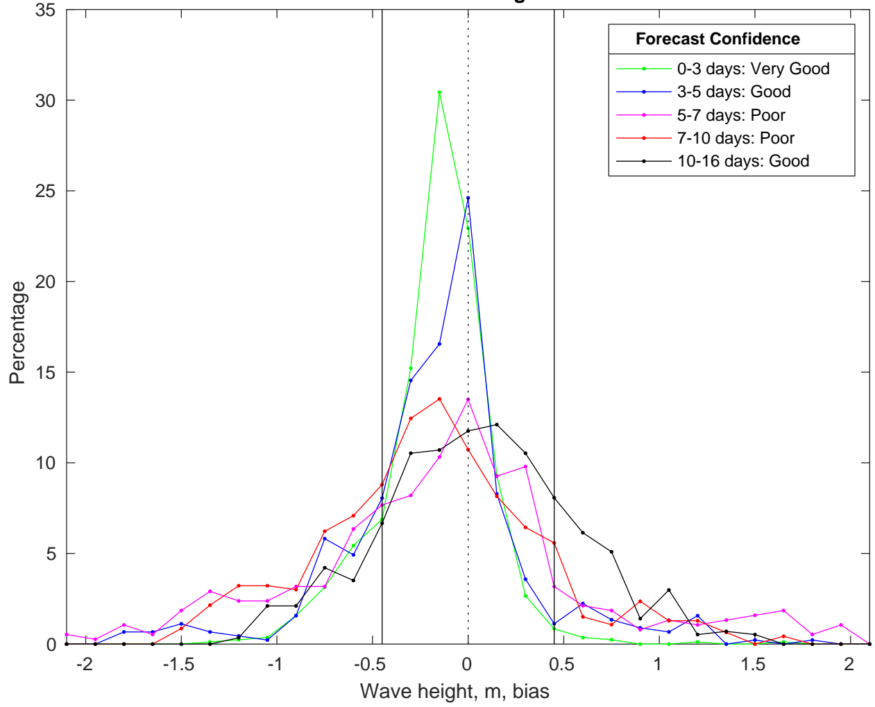
NDBC 41004 vs GFS Waves Bias Histogram: 08-Nov-2025
