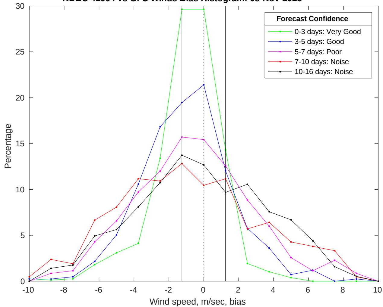
NDBC 41004 vs GFS Winds Bias Histogram: 08-Nov-2025
