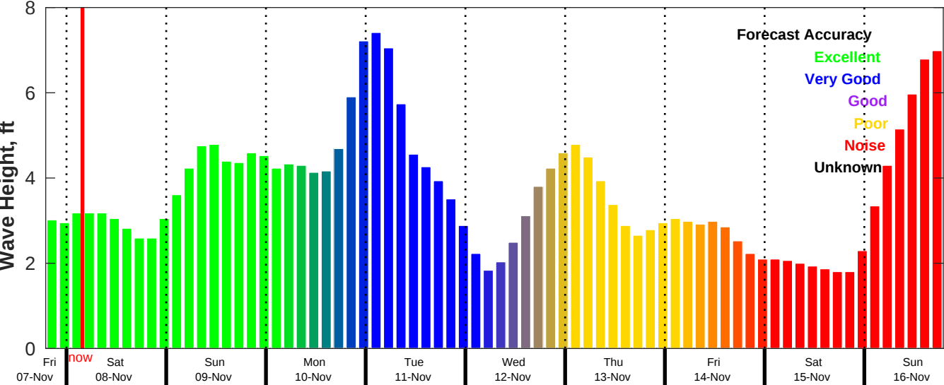
CMEMS Wave Forecast for NDBC 41004 from 07-Nov-2025 19:00:00 to 16-Nov-2025 19:00:00
