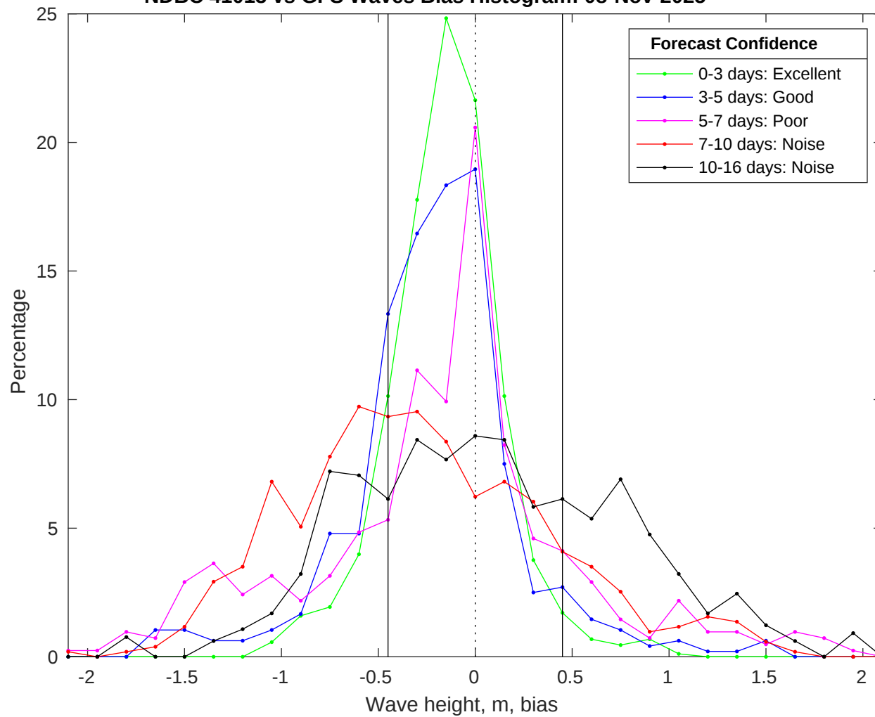
NDBC 41013 vs GFS Waves Bias Histogram: 08-Nov-2025
