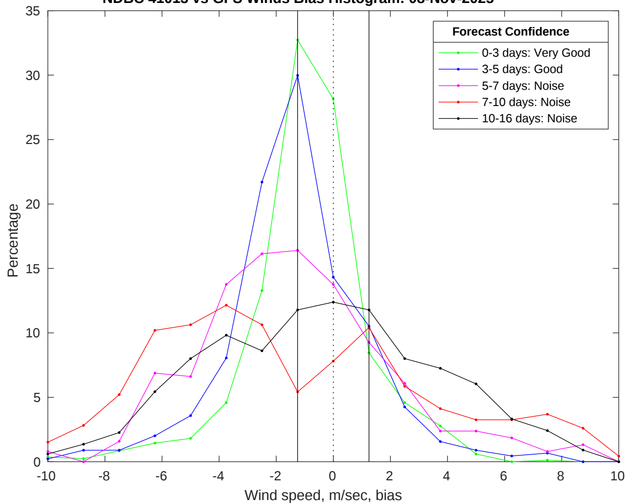
NDBC 41013 vs GFS Winds Bias Histogram: 08-Nov-2025
