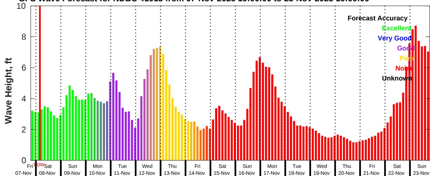
GFS Wave Forecast for NDBC 41013 from 07-Nov-2025 19:00:00 to 23-Nov-2025 19:00:00
