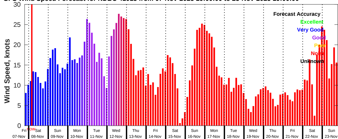
GFS Wind Speed Forecast for NDBC 41013 from 07-Nov-2025 19:00:00 to 23-Nov-2025 19:00:00
