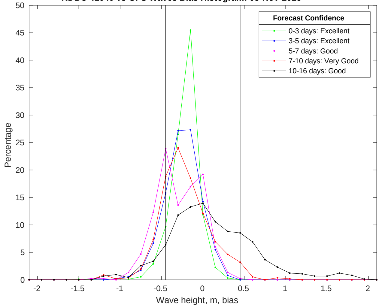
NDBC 41040 vs GFS Waves Bias Histogram: 08-Nov-2025
