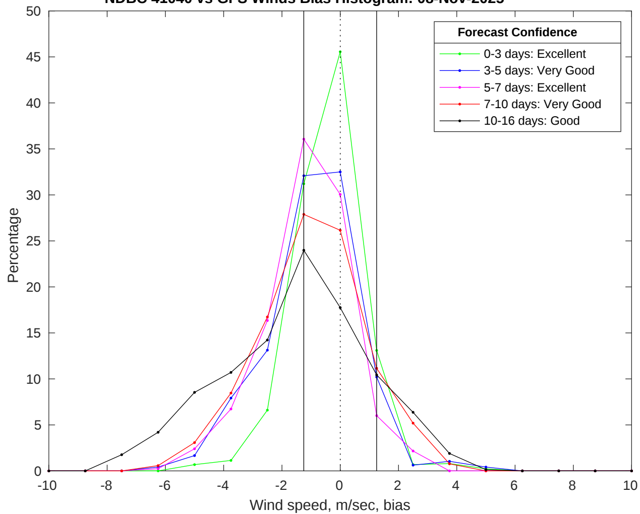
NDBC 41040 vs GFS Winds Bias Histogram: 08-Nov-2025
