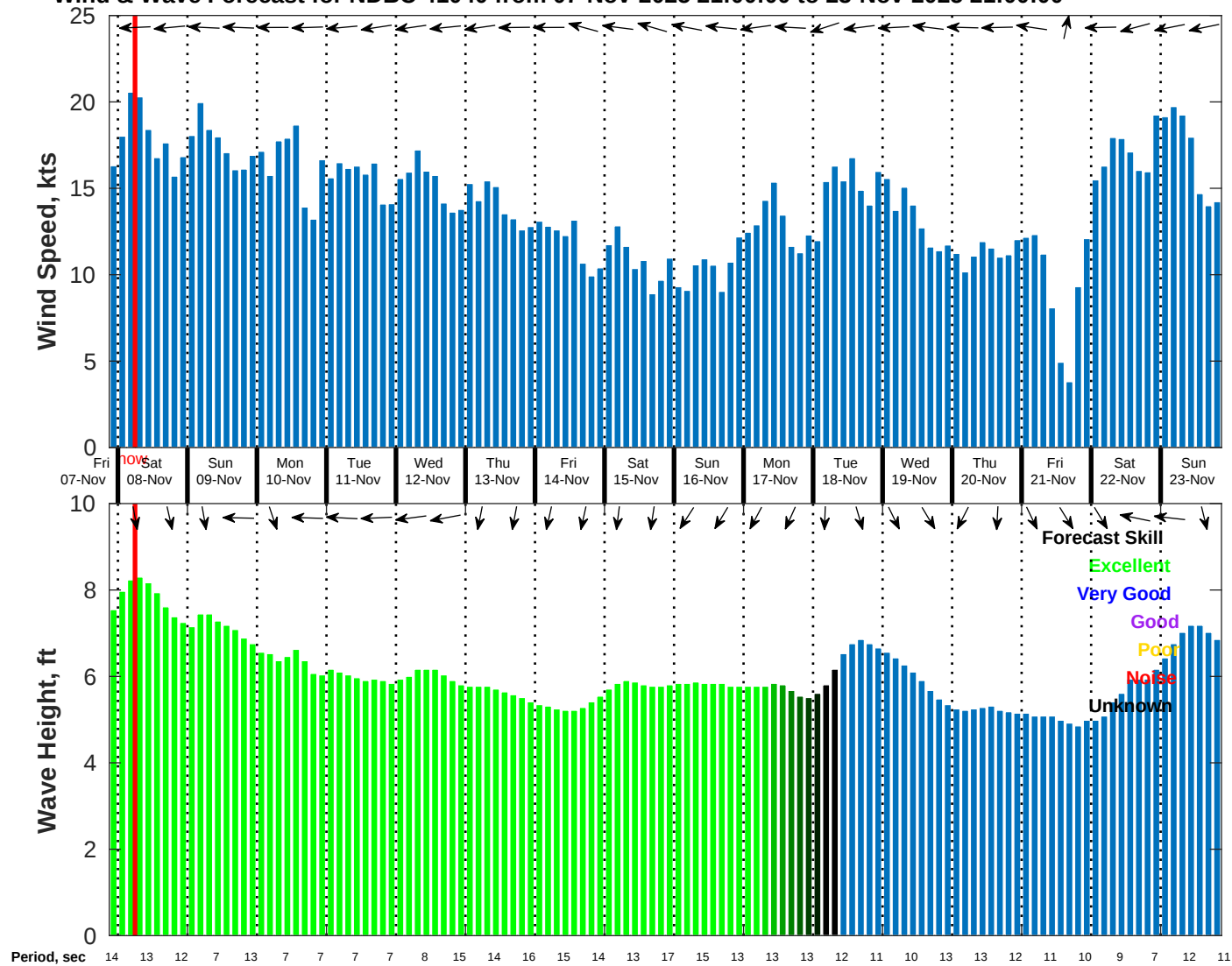
Wind & Wave Forecast for NDBC 41040 from 07-Nov-2025 21:00:00 to 23-Nov-2025 21:00:00
