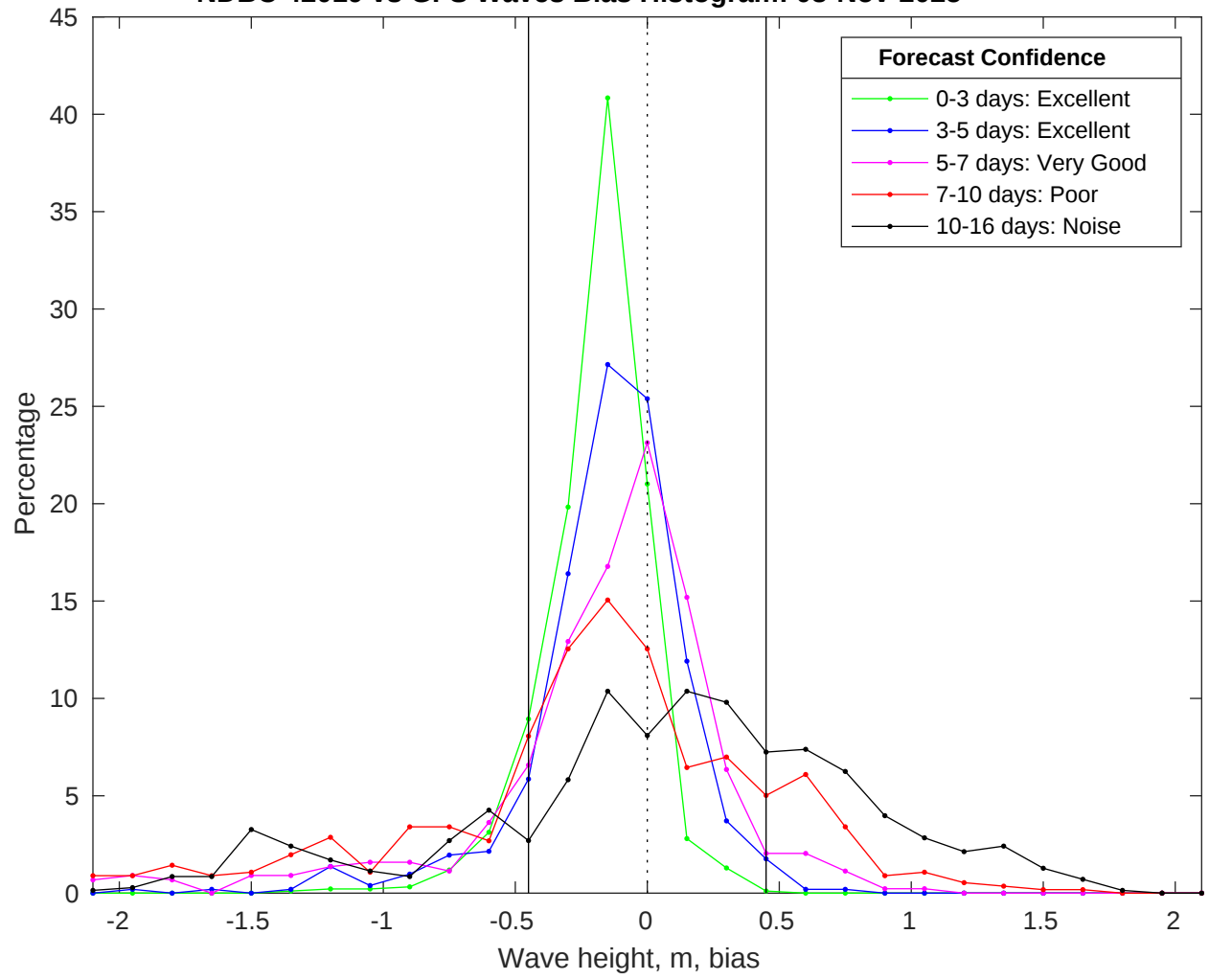
NDBC 42019 vs GFS Waves Bias Histogram: 08-Nov-2025
