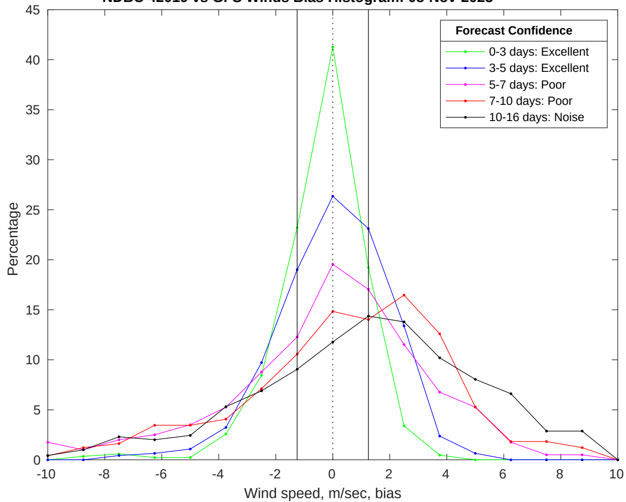
NDBC 42019 vs GFS Winds Bias Histogram: 08-Nov-2025
