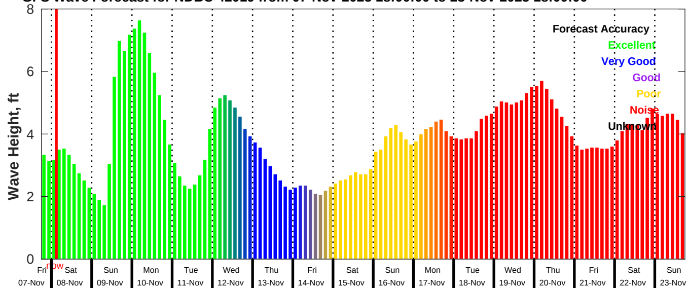
GFS Wave Forecast for NDBC 42019 from 07-Nov-2025 18:00:00 to 23-Nov-2025 18:00:00
