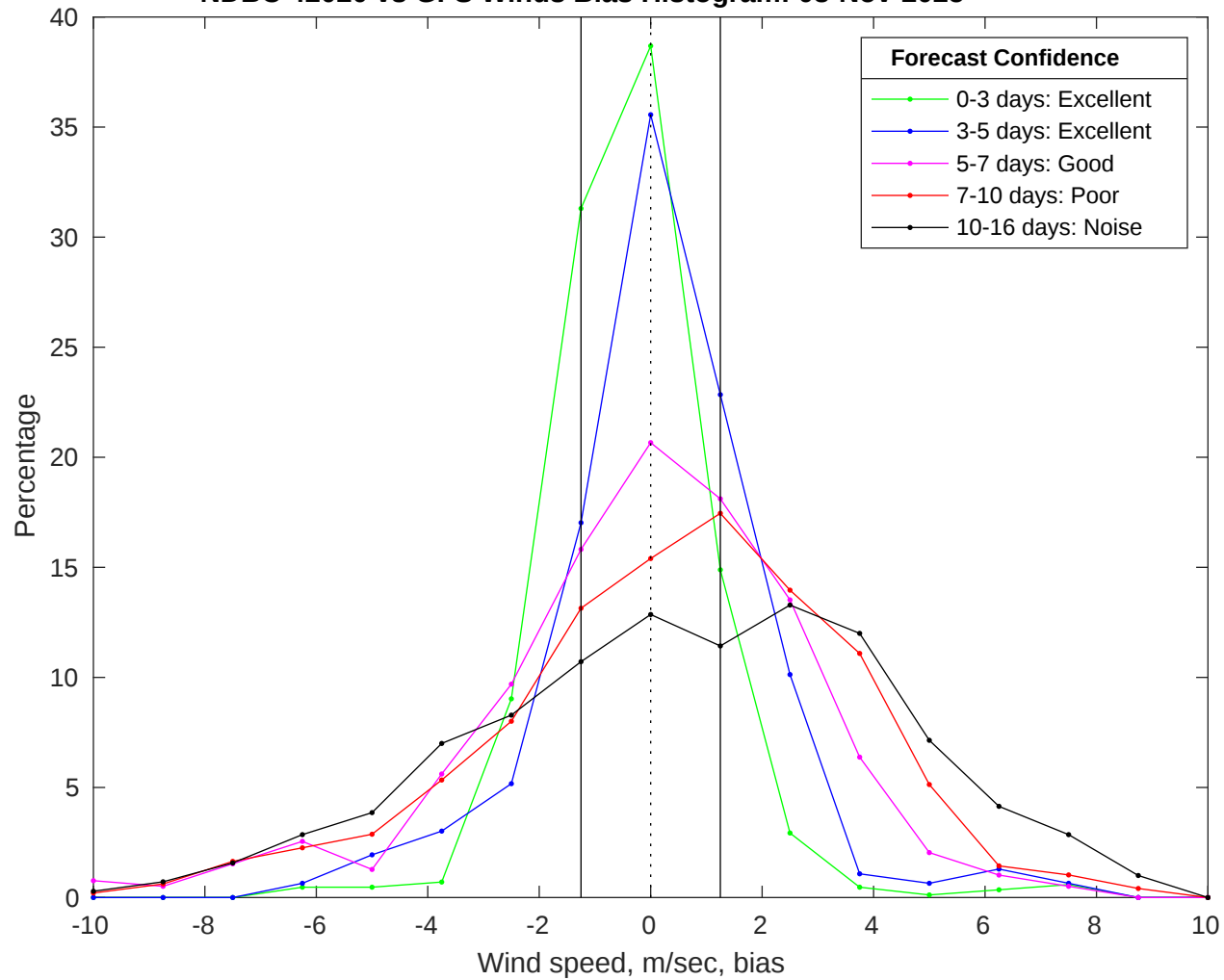
NDBC 42020 vs GFS Winds Bias Histogram: 08-Nov-2025
