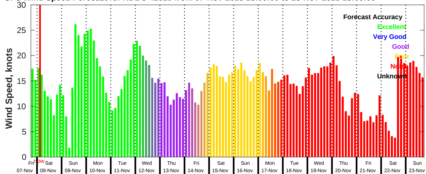
GFS Wind Speed Forecast for NDBC 42020 from 07-Nov-2025 18:00:00 to 23-Nov-2025 18:00:00
