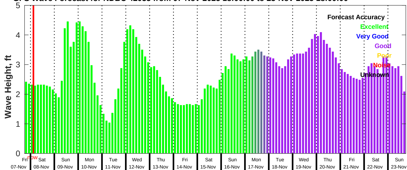
GFS Wave Forecast for NDBC 42035 from 07-Nov-2025 18:00:00 to 23-Nov-2025 18:00:00
