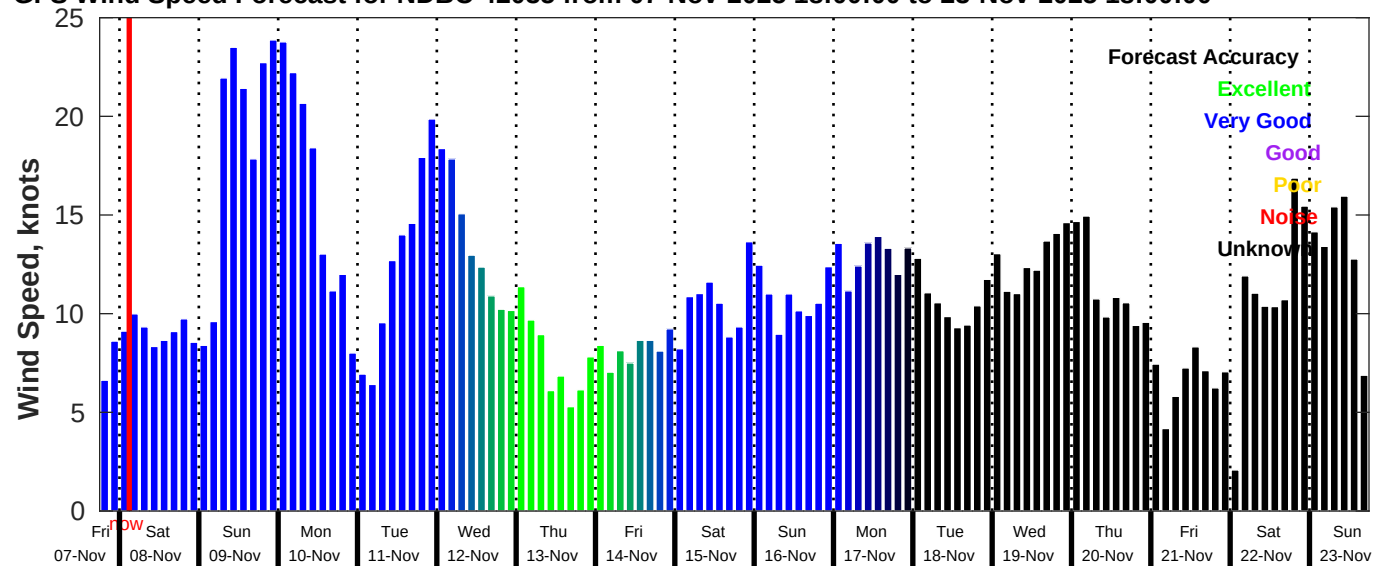
GFS Wind Speed Forecast for NDBC 42035 from 07-Nov-2025 18:00:00 to 23-Nov-2025 18:00:00
