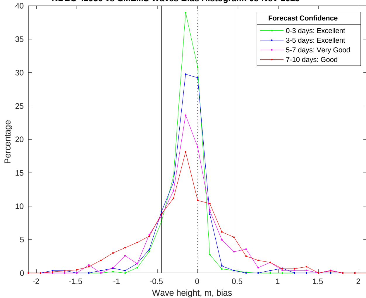
NDBC 42036 vs CMEMS Waves Bias Histogram: 08-Nov-2025
