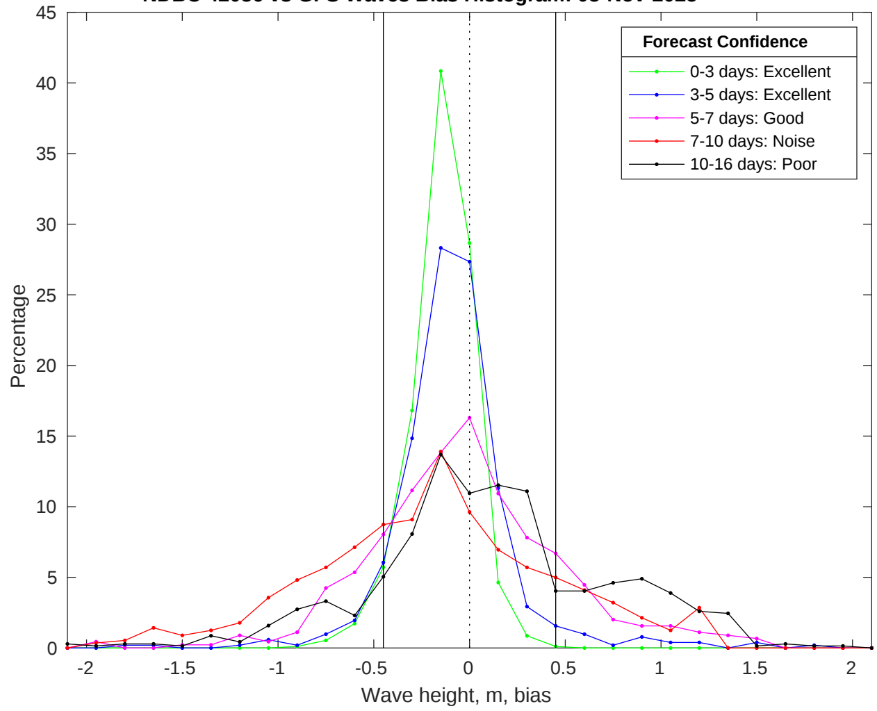
NDBC 42036 vs GFS Waves Bias Histogram: 08-Nov-2025
