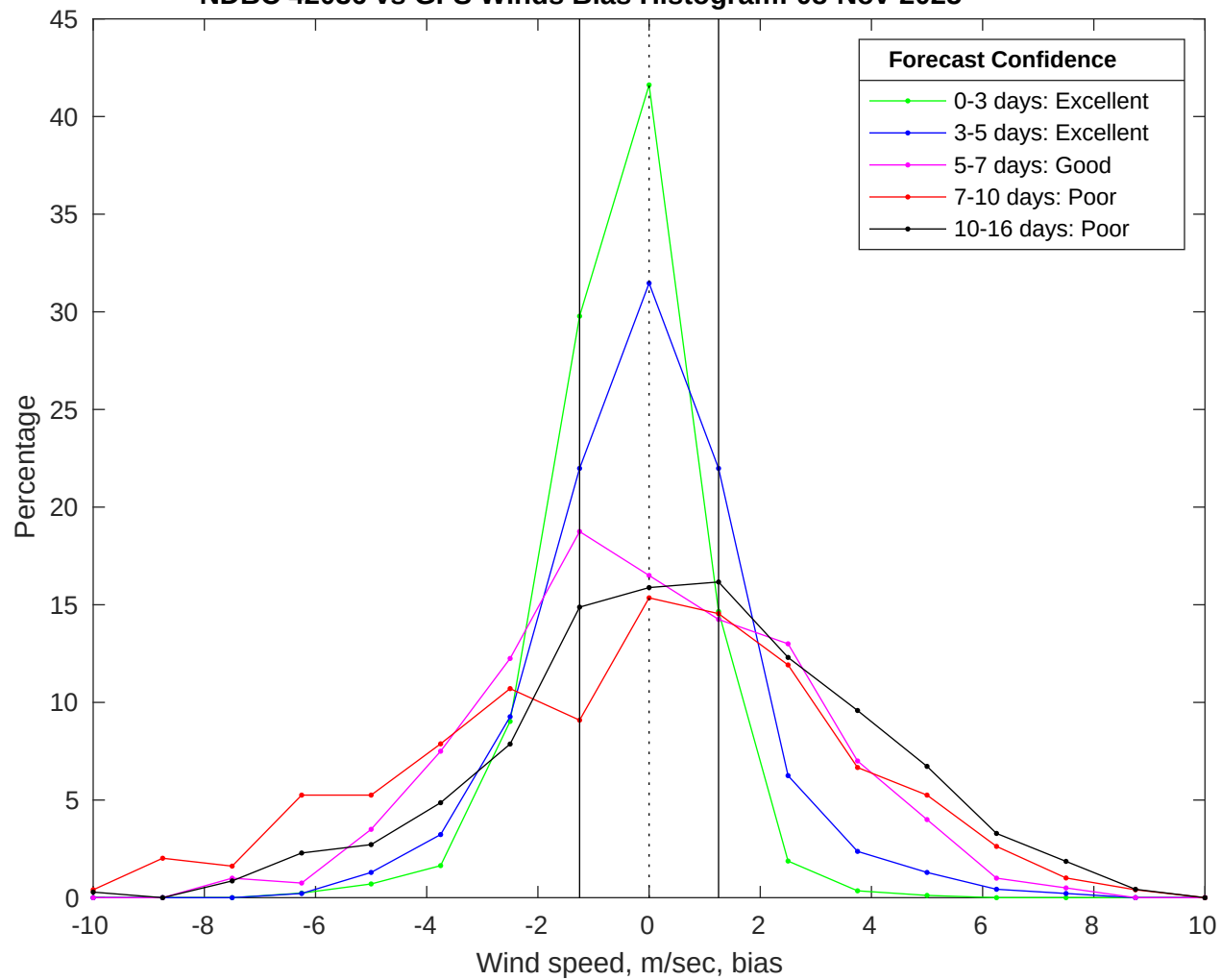
NDBC 42036 vs GFS Winds Bias Histogram: 08-Nov-2025
