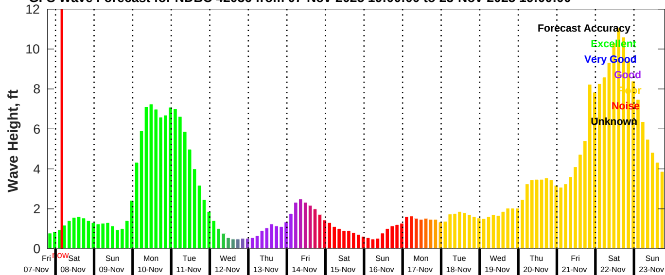
GFS Wave Forecast for NDBC 42036 from 07-Nov-2025 19:00:00 to 23-Nov-2025 19:00:00
