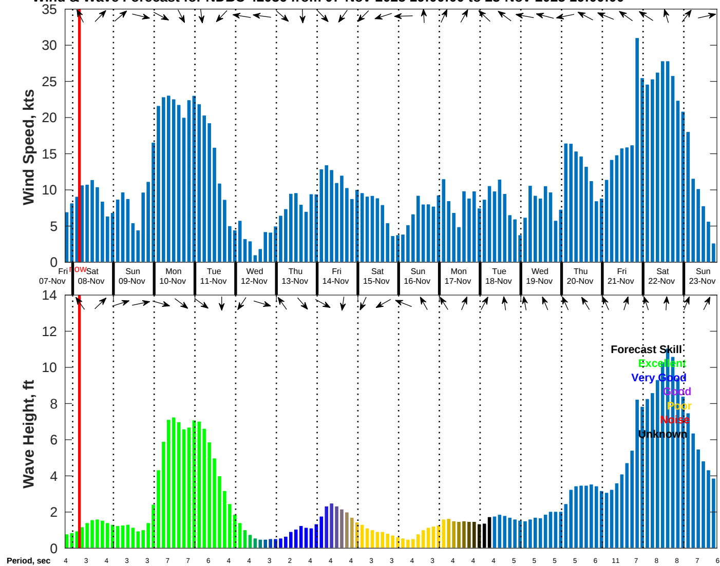
Wind & Wave Forecast for NDBC 42036 from 07-Nov-2025 19:00:00 to 23-Nov-2025 19:00:00
