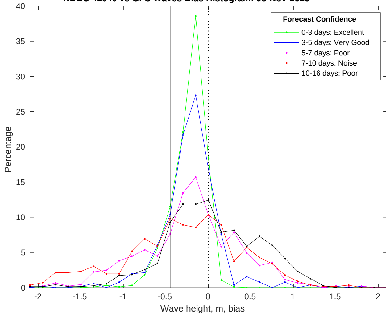
NDBC 42040 vs GFS Waves Bias Histogram: 08-Nov-2025
