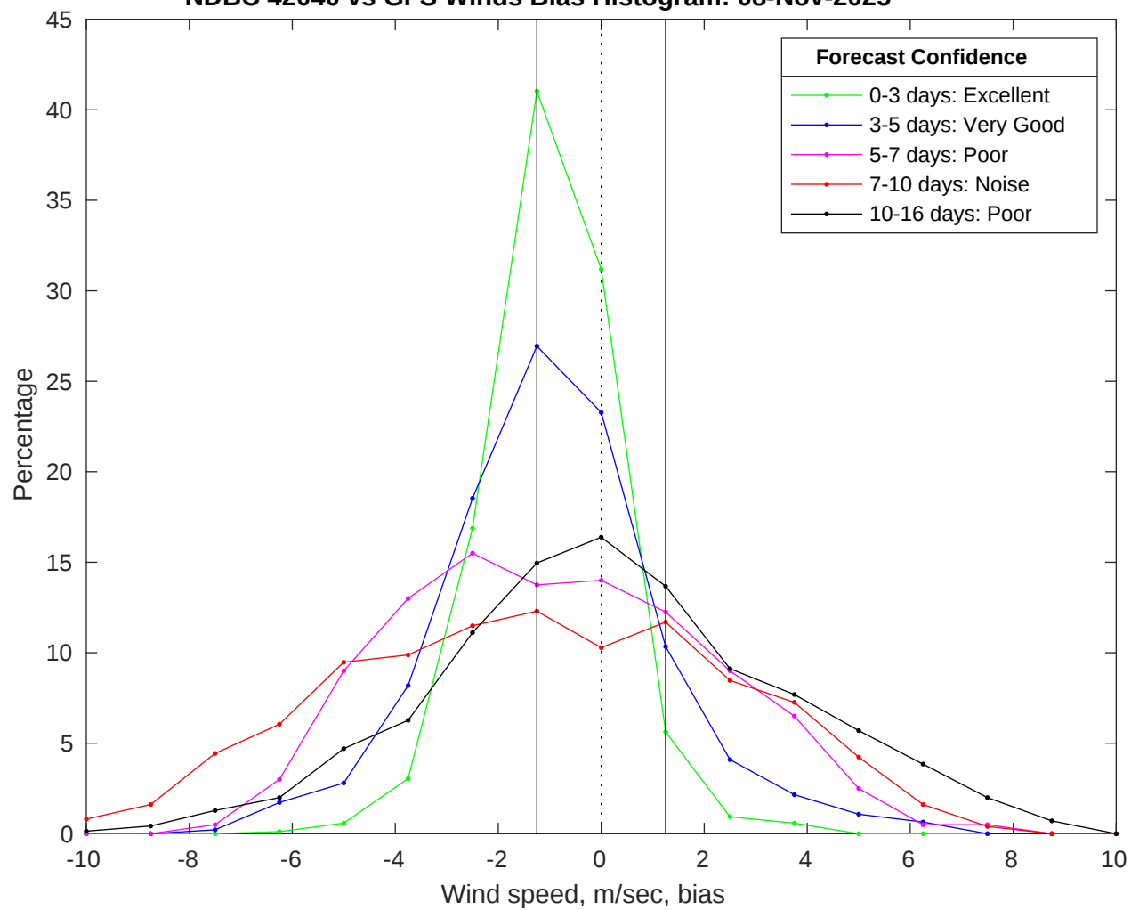
NDBC 42040 vs GFS Winds Bias Histogram: 08-Nov-2025
