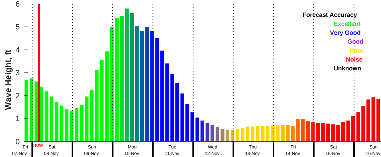
CMEMS Wave Forecast for NDBC 42040 from 07-Nov-2025 19:00:00 to 16-Nov-2025 19:00:00
