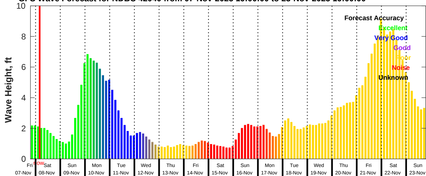
GFS Wave Forecast for NDBC 42040 from 07-Nov-2025 19:00:00 to 23-Nov-2025 19:00:00
