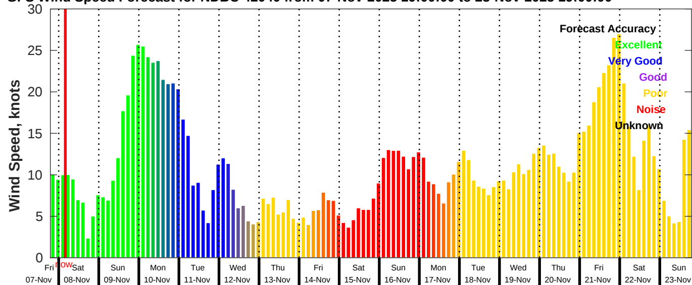
GFS Wind Speed Forecast for NDBC 42040 from 07-Nov-2025 19:00:00 to 23-Nov-2025 19:00:00
