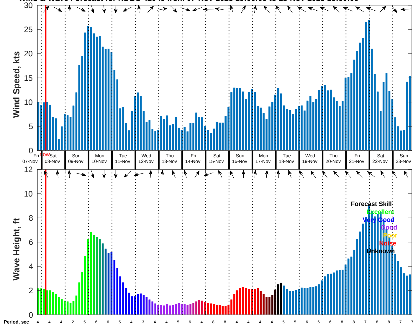
Wind & Wave Forecast for NDBC 42040 from 07-Nov-2025 19:00:00 to 23-Nov-2025 19:00:00
