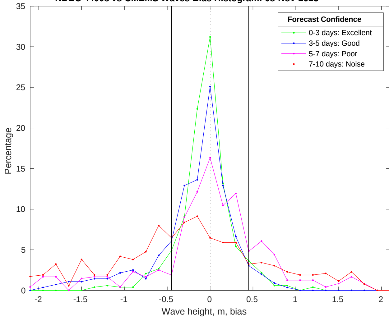
NDBC 44008 vs CMEMS Waves Bias Histogram: 08-Nov-2025
