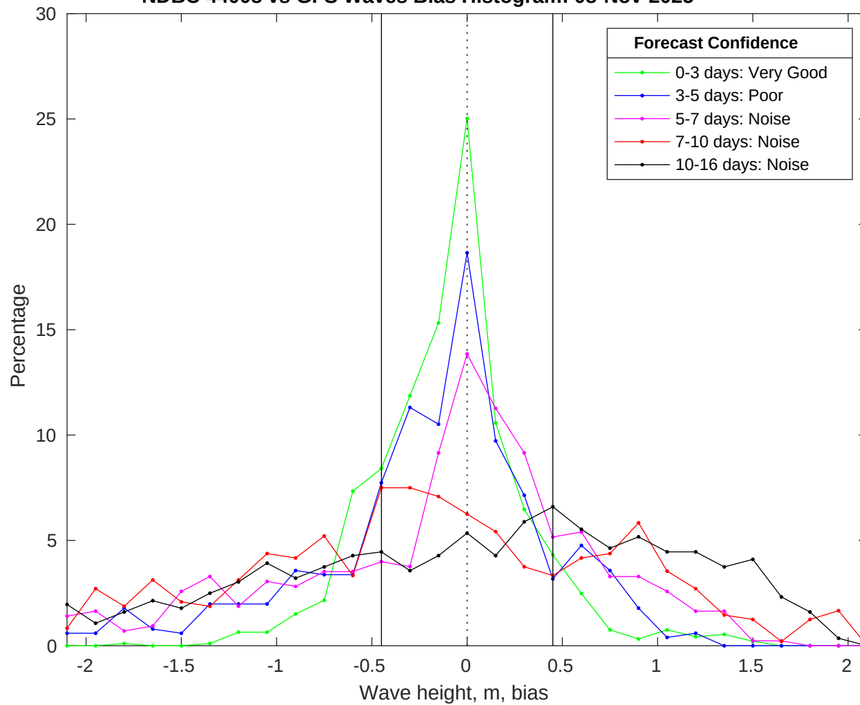
NDBC 44008 vs GFS Waves Bias Histogram: 08-Nov-2025
