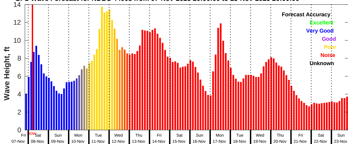
GFS Wave Forecast for NDBC 44008 from 07-Nov-2025 20:00:00 to 23-Nov-2025 20:00:00
